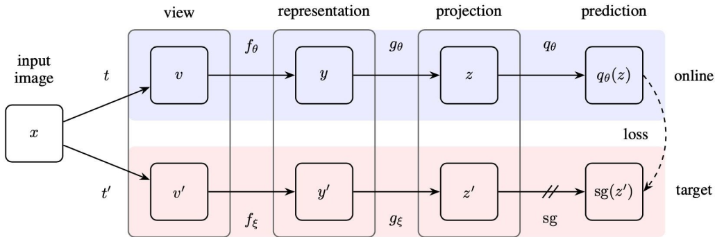
Figure 2: BYOL's architecture. BYOL minimizes a similarity loss between q_\theta(z) and \text{sg}(z') , where \theta are the trained weights, \xi are an exponential moving average of \theta and \text{sg} means stop-gradient. At the end of training, everything but f_\theta is discarded and y is used as the image representation.
